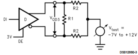
FIGURE 5. V_{OD3}
