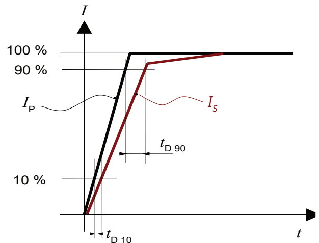
Figure 6: t_{D10} (delay time @ 10 %) and t_{D90} (delay time @ 90 %)
