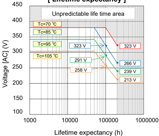
[ Lifetime expectancy ]
