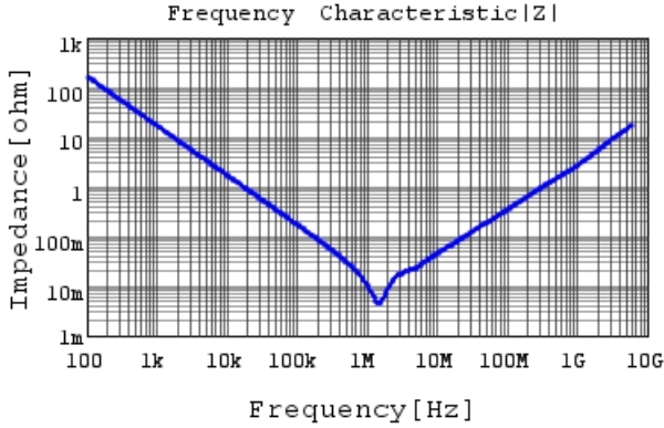
GRM31CR61C106KA88 |Z| DCOV,25degC
