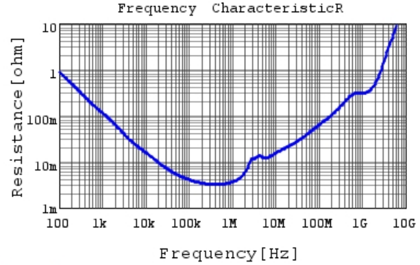
GRM31CR61C106KA88 R DCOV,25degC
