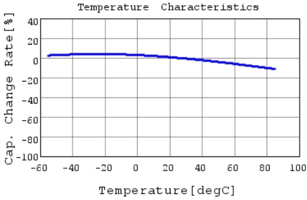
GRM31CR61C106KA88 C-Temp. capchange, DC0.0V,
