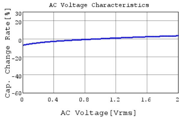
GRM31CR61C106KA88 C-AC Voltage capchange, Dc
