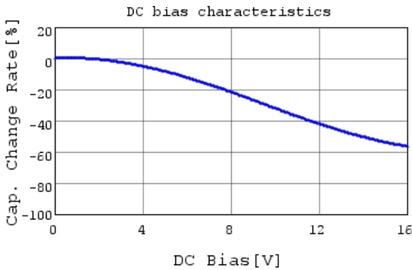
GRM31CR61C106KA88 C-DC bias capchange, 25.0c
