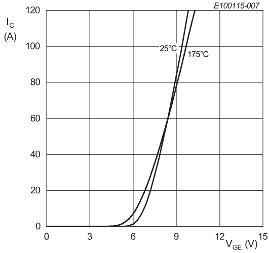
Fig. 7. Typical transfer characteristic
