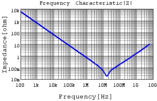
GRT155R61C474KE01 |Z| DCOV, 25degC
