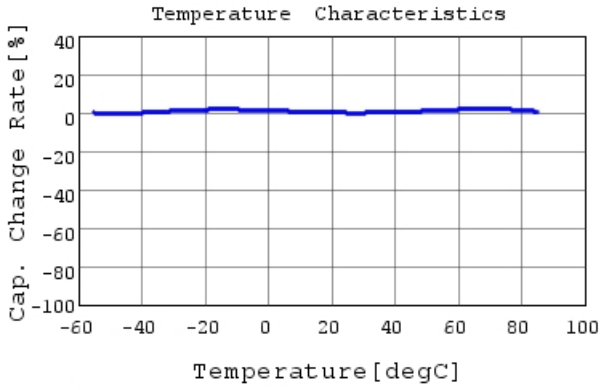
GRT155R61C474KE01 C-Temp. capchange, DC0.0V,
