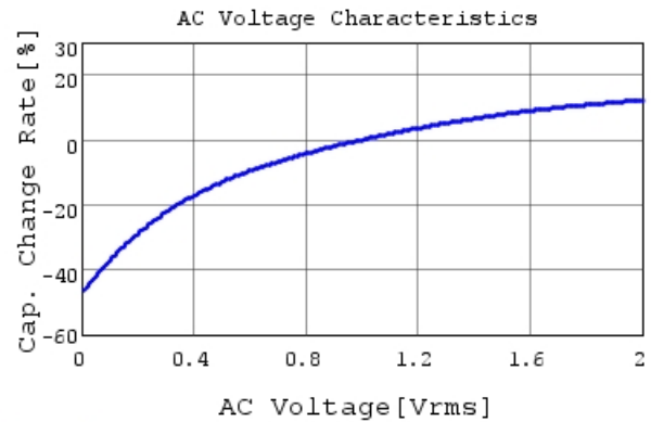
GRT155R61C474KE01 C-AC Voltage capchange, Dc
