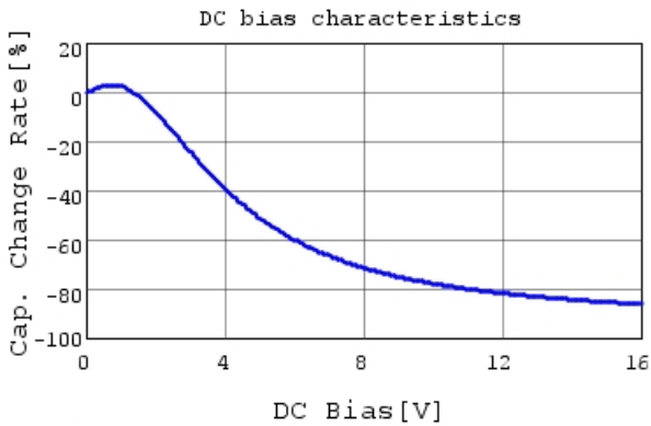
GRT155R61C474KE01 C-DC bias capchange, 25.0c
