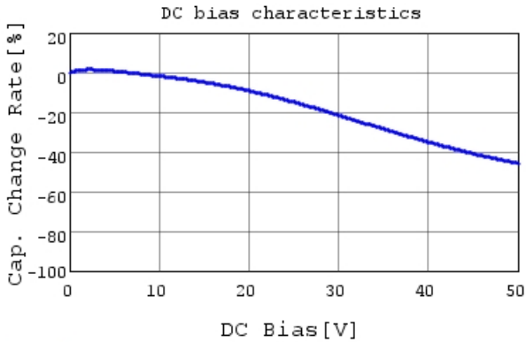
GRM155R71H222JA01 C-DC bias capchange, 25.0c
