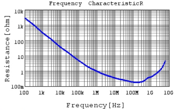
GRM155R71H222JA01 R DCOV, 25degC
