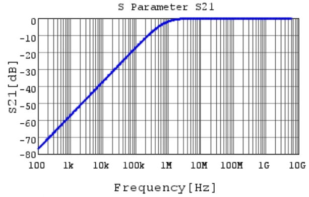
GRM155R71H222JA01 S21 DC0V, 25degC
