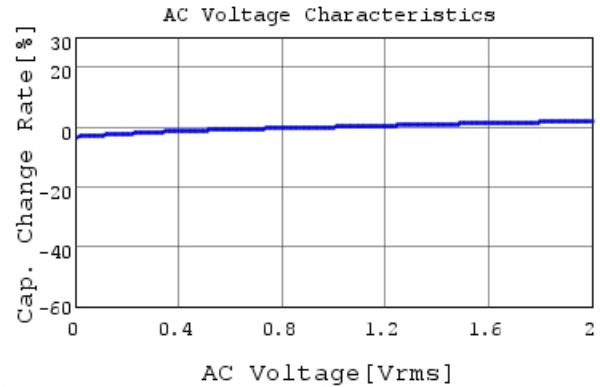
GRM155R71H222JA01 C-AC Voltage capchange, Dc
