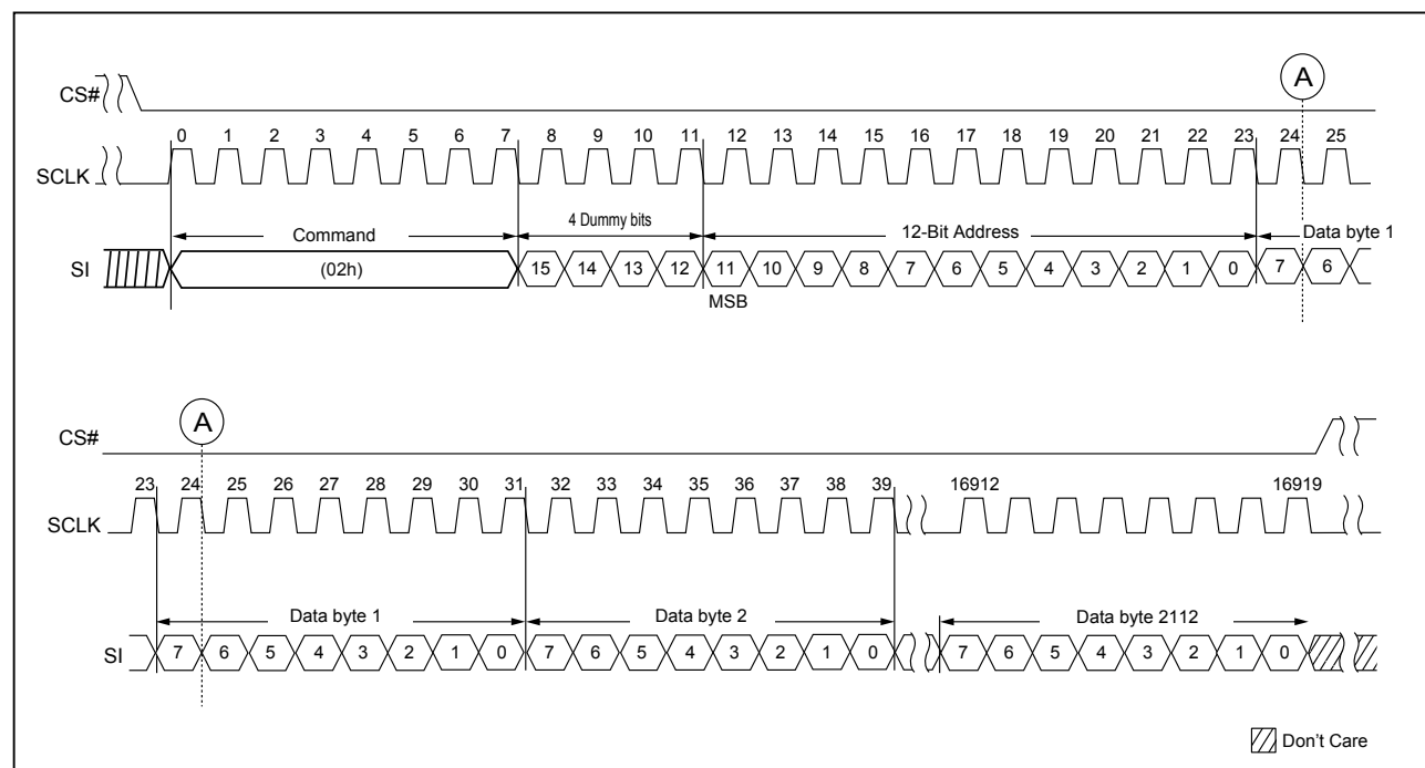
Figure 25. PROGRAM LOAD (02h) Timing
