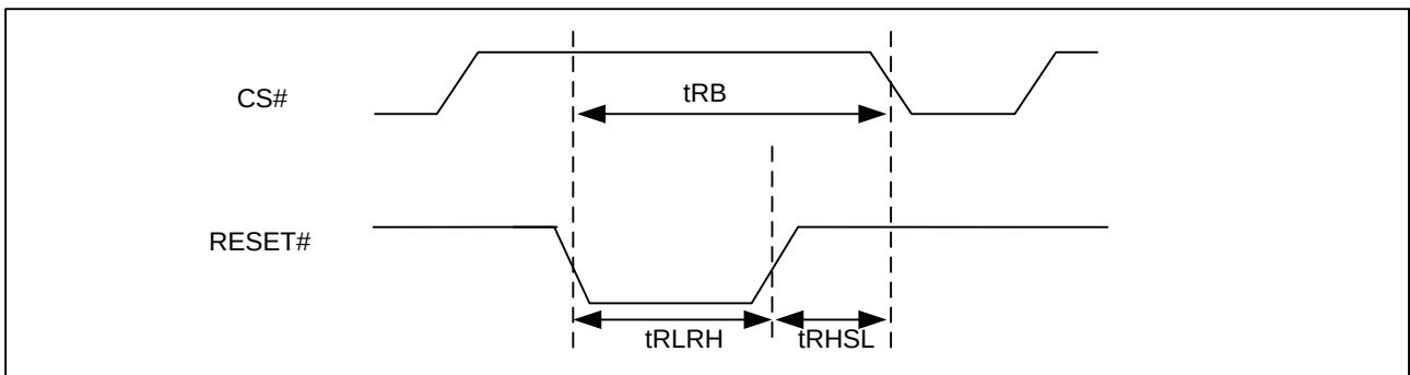
Figure 76 RESET Timing
