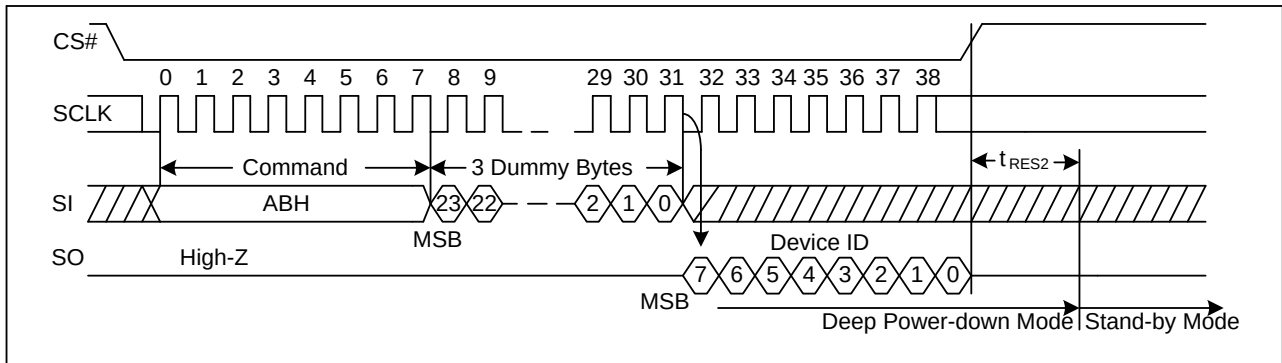
Figure 55 Release Power-Down/Read Device ID Sequence Diagram
