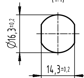
panel cut out (1:1)
