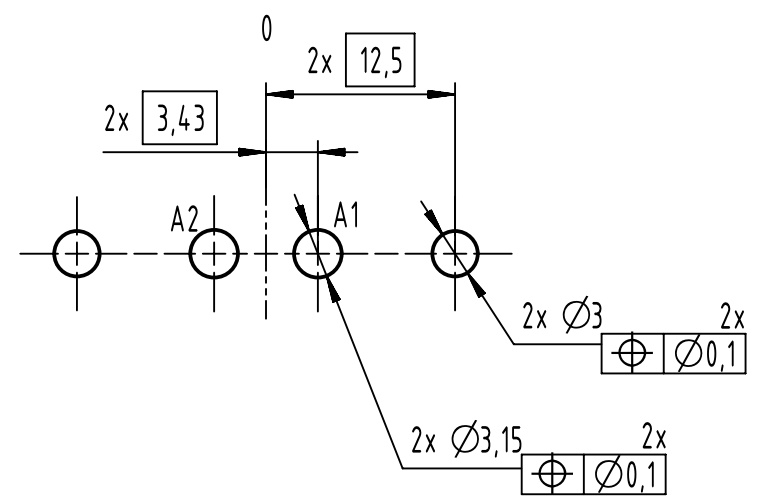
PCB hole pattern, mounting side
