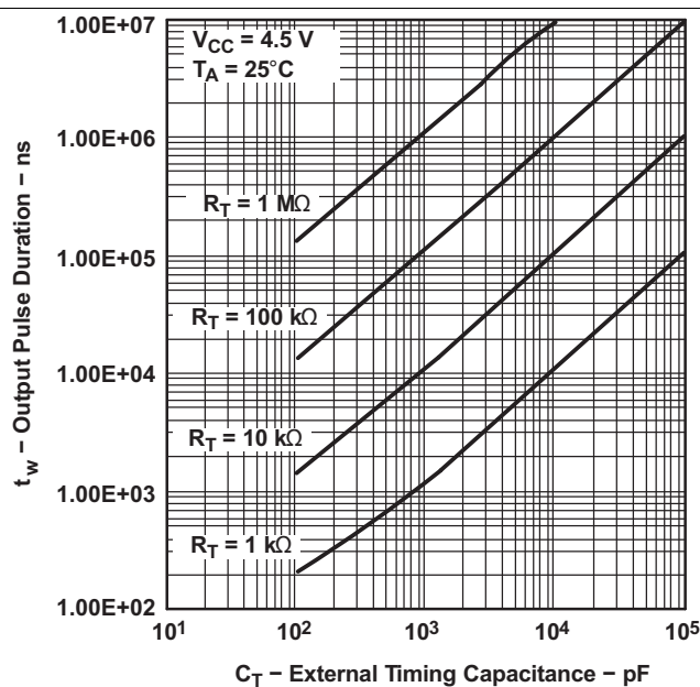
Figure 13. Output Pulse Duration vs. External Timing Capacitance
