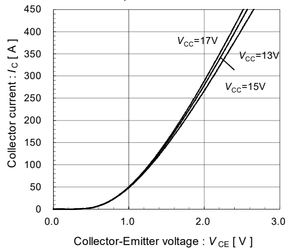
Collector current vs. Collector-Emittor voltage (typ.) T_{vj}=125^{\circ}\text{C} [ Terminal ]
