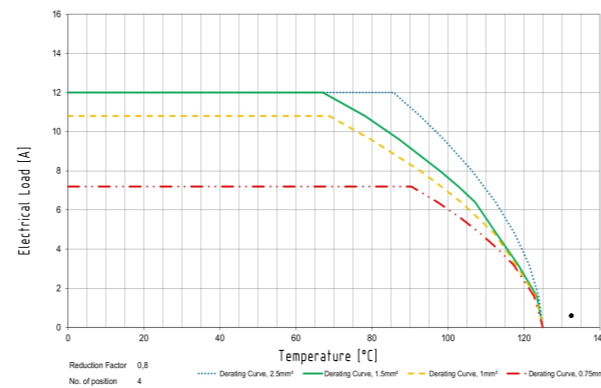
Derating: har-flexicon 5.00/5.08 MTV:
