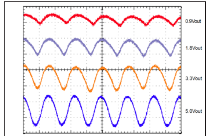
Figure 16: Output Voltage Ripple at nominal input voltage and rated load current (50 mV/div). Load capacitance: 22\ \mu\text{F} ceramic cap. Bandwidth: 20 MHz. See Figure 13.
