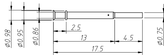
Bushing
