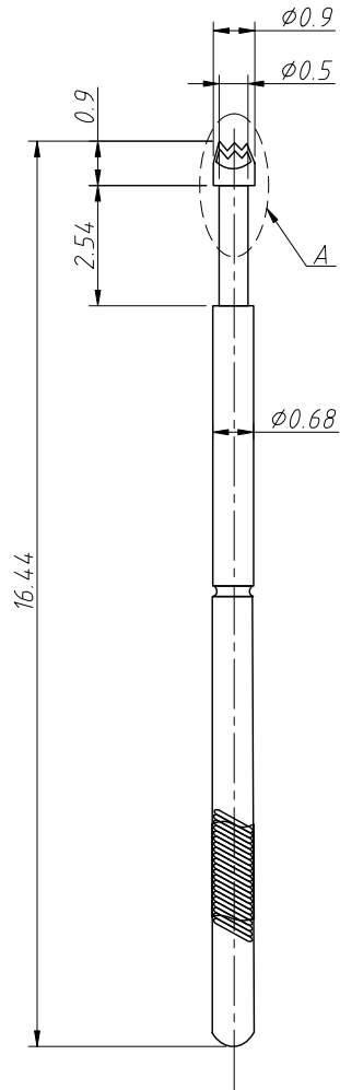
Needle Bar
