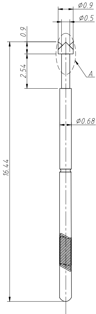
Needle Bar
