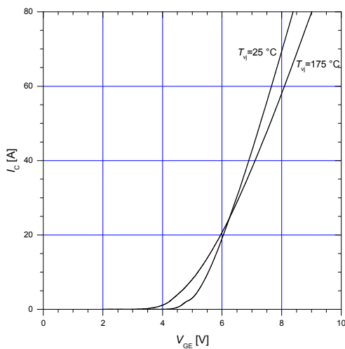
Graph 5 Typical transfer characteristics V_{CE} = 20\text{ V}
