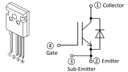
TO-247-4-P2
