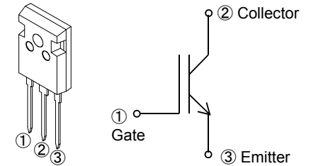
TO-247-P/TO-247-P2
