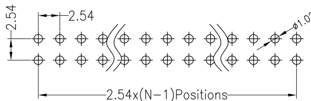
Recommended P.C.B Layout(Top Side) (PCB BOARD TOLERANCE±0.05)
