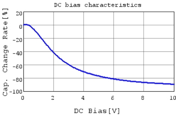
GRT155R61A225KE01 C-DC bias capchange, 25.0c
