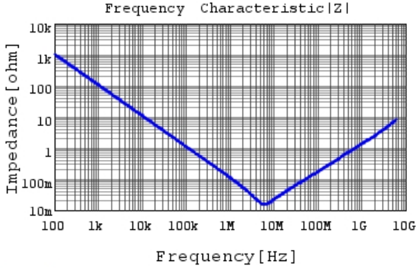
GRT155R61A225KE01 |Z| DCOV, 25degC
