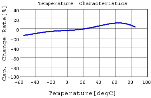
GRT155R61A225KE01 C-Temp. capchange, DC0.0V,
