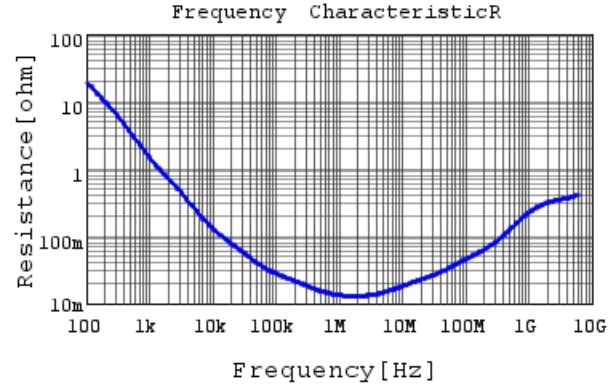
GRT155R61A225KE01 R DCOV, 25degC
