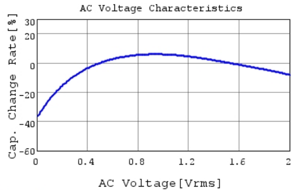
GRT155R61A225KE01 C-AC Voltage capchange, Dc
