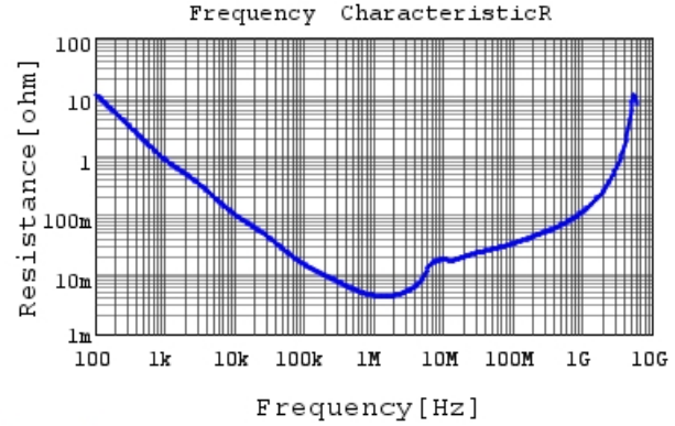
GRM21BR61H475KE51 R DCOV, 25degC
