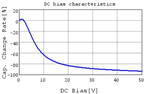
GRM21BR61H475KE51 C-DC bias capchange, 25.0c
