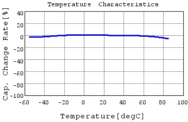
GRM21BR61H475KE51 C-Temp. capchange, DC0.0V,
