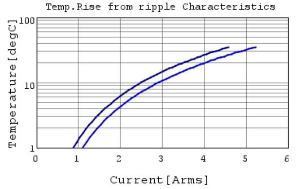
GRM21BR61H475KE51 Temp.rise — 500kHz
