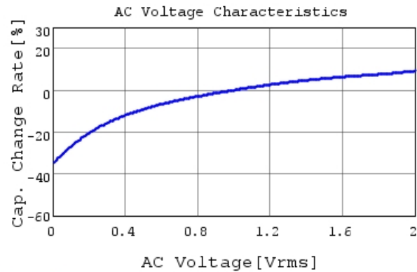
GRM21BR61H475KE51 C-AC Voltage capchange, DC
