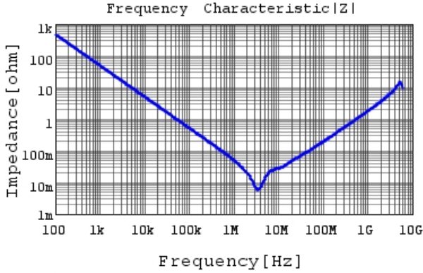
GRM21BR61H475KE51 |Z| DCOV, 25degC
