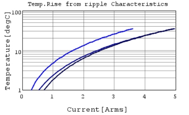
GRM188R61C106MA73 Temp.rise — 80kHz
