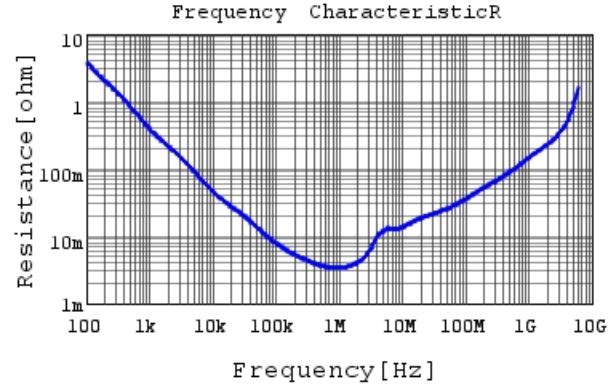
GRM188R61C106MA73 R DCOV,25degC
