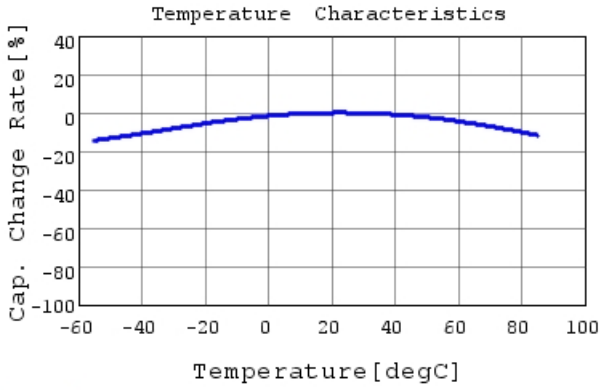
GRM188R61C106MA73 C-Temp. capchange, DC0.0V,
