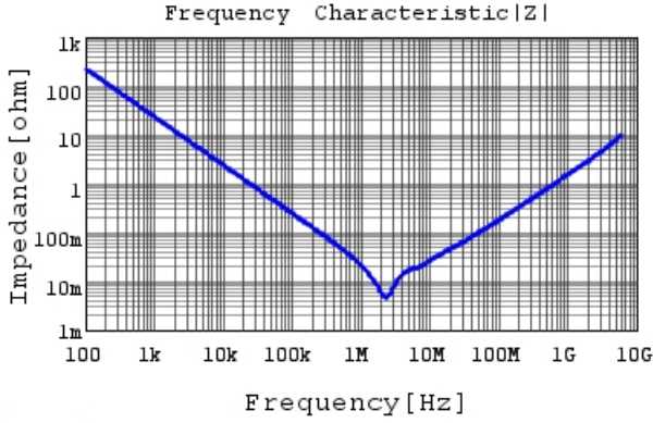
GRM188R61C106MA73 |Z| DCOV,25degC
